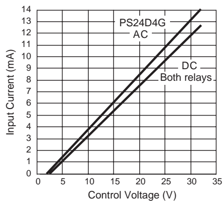
Figure 4 — PS relays
